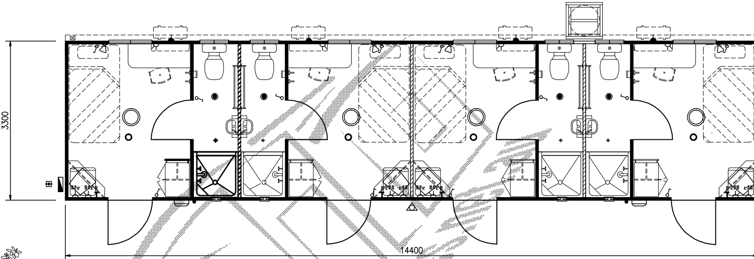
FLOOR PLAN
